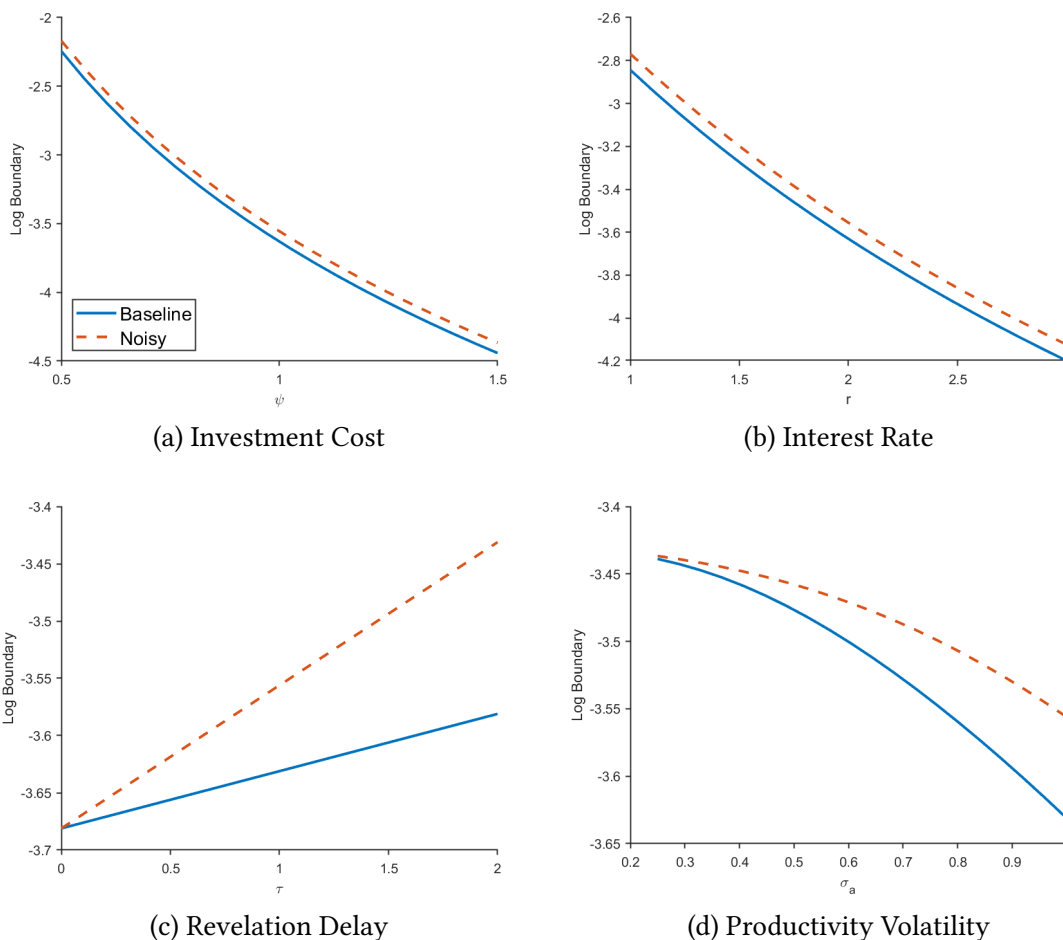
Figure 1: How the Boundary \hat{b} Depends on Various Parameters
